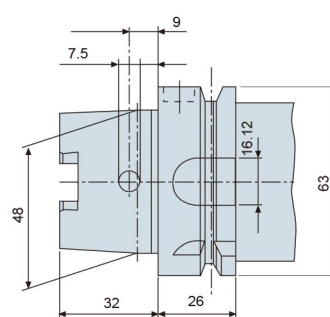
HSK A63
