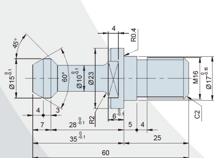
BT-40
